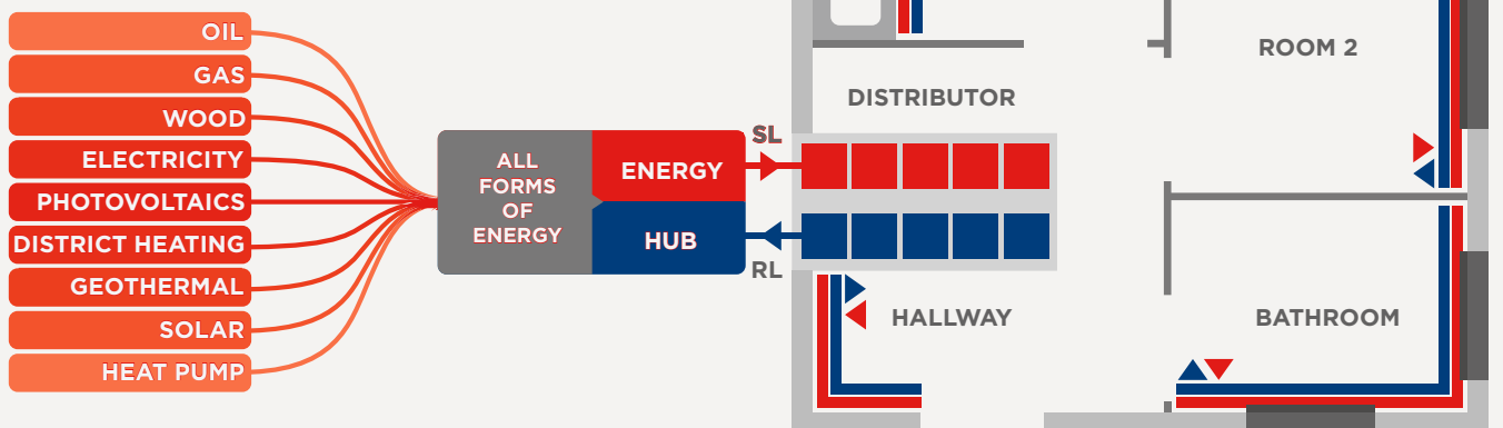
Installation example
